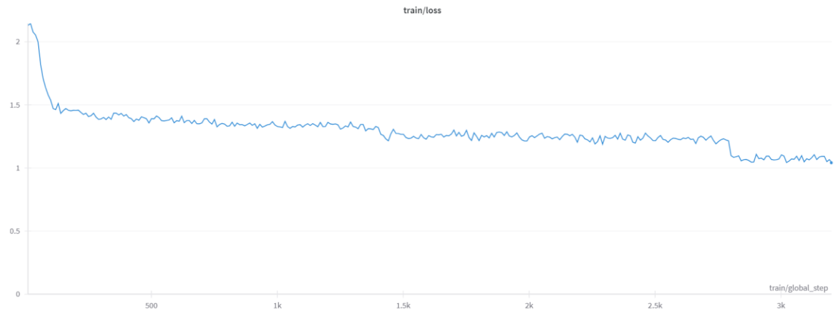
Figure 5: FALCON loss graph, Spanish instructions LoRA
