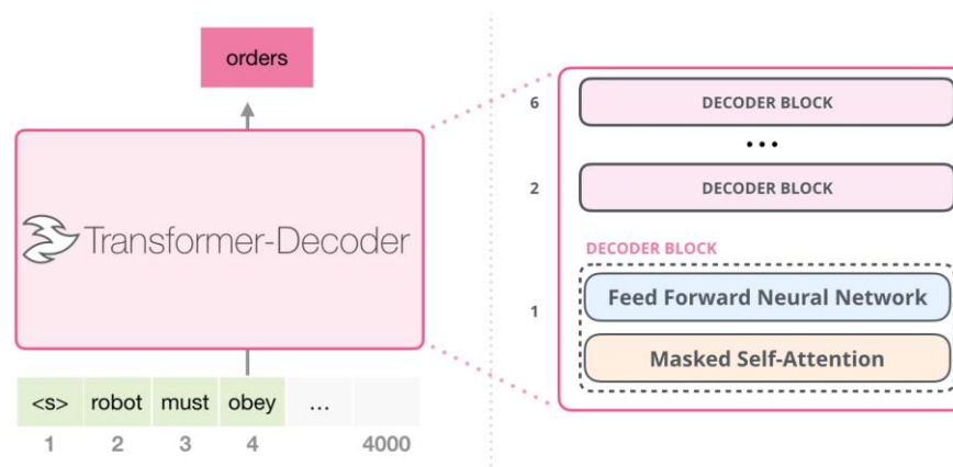
Figure 2: architecture of a decoder-only transformer model
