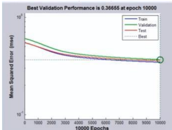
Fig. 16: Mean Squared Error of our program. In the graph we can see what modifies the performance function of the network (the error measure that minimizes the training process). By including the values of the weights and trends, the regularization produces a network that works well with the training data and offers a more fluid behavior when presented with new data.
